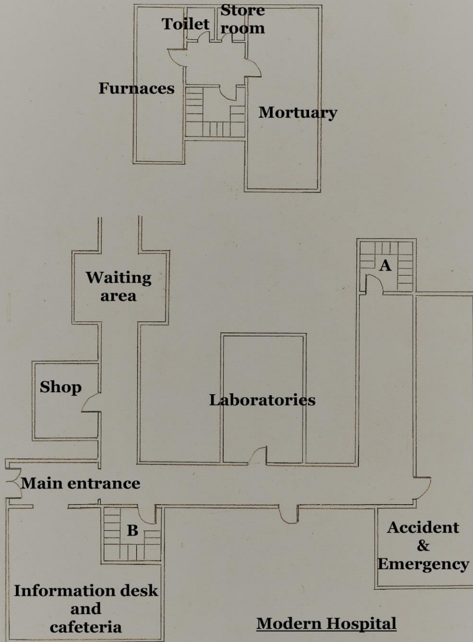
Ground Floor and Basement
